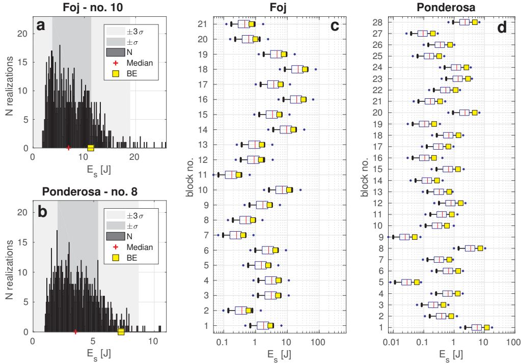
Figure 6. Seismic energy ( E_s ) result after 1000 realizations varying Q , c_R and \rho for the ground surface (see Sect. 2.1.1). a, b: both histograms (Foj, block 10, and Ponderosa, block 8), represent a randomly selected example for each quarry displaying the result for a particular block and according to the legend. c, d: boxplots indicating the median (red line), 25 th and 75 th percentiles (blue box), 5 th and 95 th percentiles (black whiskers), and full range (small blue stars) of the randomized calculation for each block at Foj and Ponderosa, respectively. Our best estimate (BE) is depicted with a yellow square.
