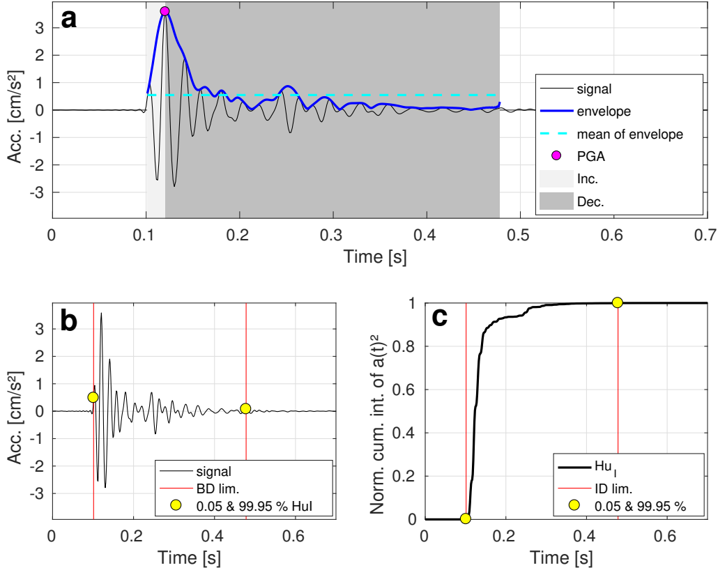
Figure 5. Time analysis of Block 4 at Foj. a: acceleration signal and amplitude envelope (computed as in Eq. 3), its mean, PGA, and duration of increasing and decreasing phases for the computation of ID (shaded in grey according to the legend). b: Acceleration signal and BD limits. c: Husid plot showing the cumulative integral of the squared acceleration and its 0.05 and 99.95% values which were used throughout the paper to determine signal duration. The integral is normalized to the maximum value.
