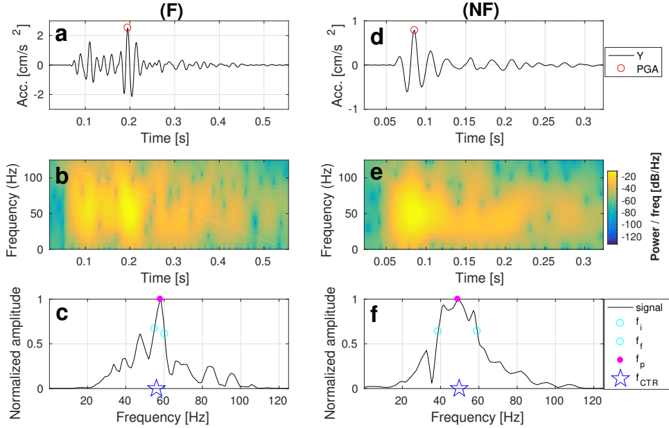
Figure 4. Accelerogram, acceleration spectrogram and acceleration spectrum (top to bottom) of a fragmentation (a, b, c) and non-fragmentation (d, e, f) impact, both recorded at Foj (blocks 1 and 7, respectively). The signal and spectra (panels a, d and c, f) were filtered between 5 and 120 Hz. The spectrograms were calculated with a moving window of length \sim 10\% that of the signal and \sim 90\% of overlap. We show the power spectral density (PSD) relative to the plotted frequencies over time (raw signal), and report it in dB as: Amplitude (dB) = 10 \log_{10}(PSD) . Central panels: note that the left-side spectrogram is centered at higher frequencies than the one to its right. Lower panels: spectral centroid f_{CTR} , predominant frequency f_p and bandwidth (represented here using initial and final points f_i and f_f ). Single-sided spectra were computed using a fast Fourier transform algorithm and amplitudes were normalized to the maximum. See text in Sect. 2.1.2 for descriptions of parameter calculations.
