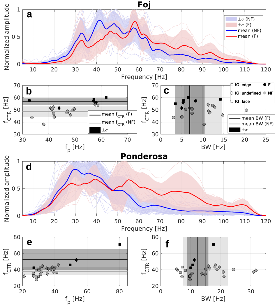
Figure 10. Analysis of fragmentation in the frequency domain. Panels a, d show a stack (mean) of all acceleration spectra and their standard deviation ( \pm\sigma ), superposed on all spectra. Means and standard deviations are computed at each plotted frequency sample. Spectra are normalized with respect to their maximum amplitude value. NF data are blue and F are red. Panels b, c, e, f show the predominant frequency, f_p , the frequency centroid, f_{CTR} , and bandwidth, BW (see Sect. 2.1.2 for definitions). Means and standard deviations are provided for f_{CTR} and BW . The marker's edge type corresponds to impact geometry (IG), as determined from the video analysis for each of the released blocks; undefined is indicated when IG could not be determined from the video analysis. Color differentiates F and NF blocks.
