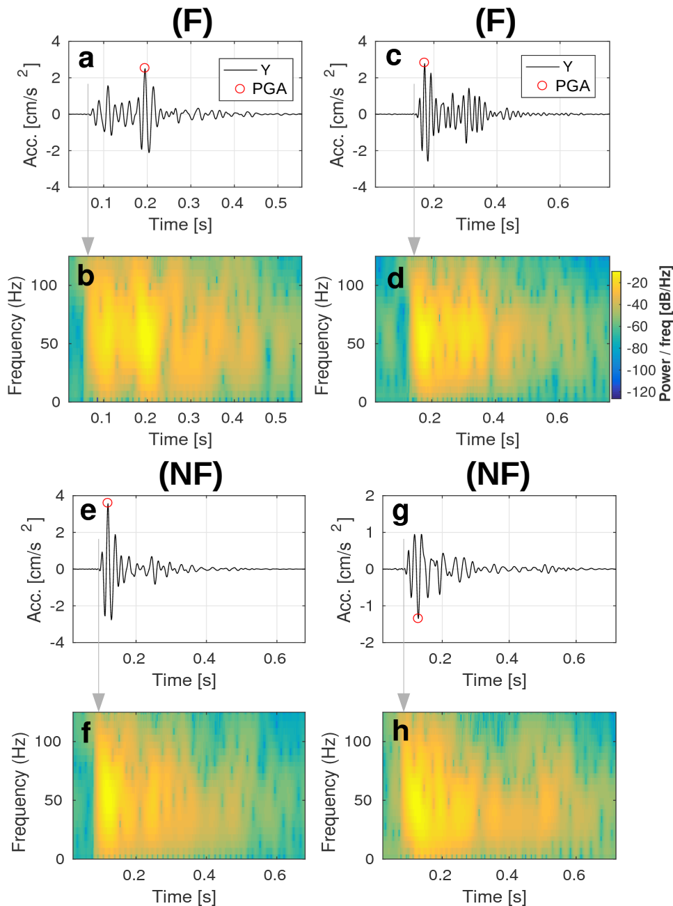
Figure 3. Accelerograms (a, c, e, g) and acceleration spectrograms (b, d, f, h) corresponding to the main ground impact of blocks 1, 3 (F) and 4, 9 (NF) at the Foj test site. Each block has its own pair (e.g. a, b for block 1, c, d for block 3, and so on), and arrows are provided to help correlate the start times of the signal and the energy displayed in the spectrograms. The most energetic frequencies were those around 50 Hz (slightly higher for F impacts), although the frequency band 5-120 Hz was filled to some extent for most of the impacts. The spectrograms were calculated with a moving window of length \sim 10\% that of the signal and \sim 90\% of overlap. They present the power spectral density (PSD) relative to the shown frequencies over time, and are reported in dB as: Amplitude (dB) = 10 \log_{10}(PSD) . In addition, no filtering is applied before displaying the spectrograms, because they were used as a tool for deciding which passband should be kept.
