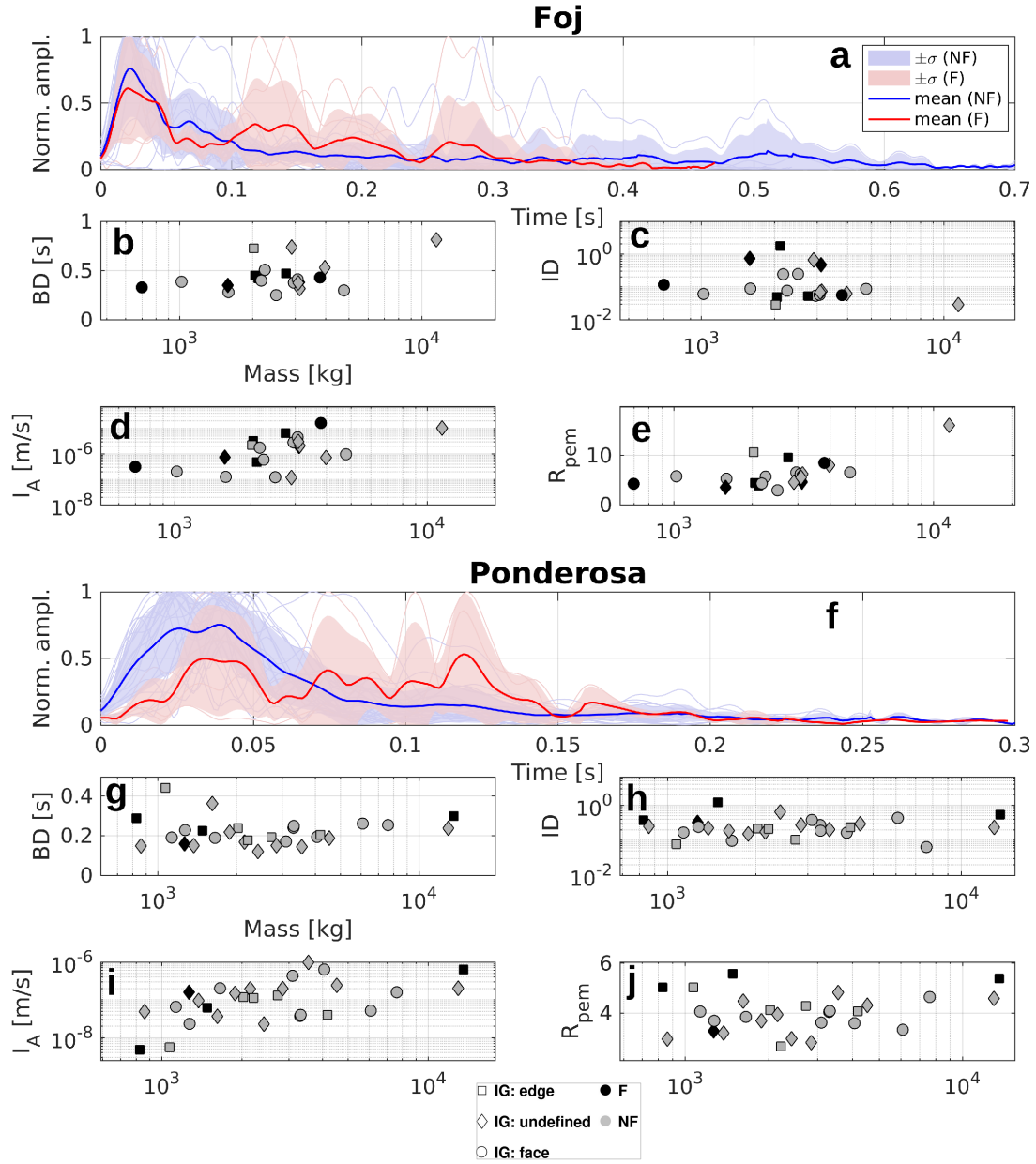
Figure 11. Analysis of fragmentation in the time domain. Panels a, f show a stack (mean) of all envelopes (computed as in Eq. 3 for the maximum component; here, envelopes are also normalized to the maximum value of each event), and their standard deviation reach ( \pm\sigma ), superposed on all envelopes. Means and standard deviations are computed for each plotted time sample. NF data are blue and F are red. Parameters shown in panels b, c, d, e, g, h, i, j are the bounded duration (BD), increasing/decreasing time ratio (ID), arias intensity ( I_A ), and ratio of the envelope peak to the envelope mean ( R_{pem} ) (see Sect. 2.1.2 for definitions). Mass is displayed along the X axes of these plots. The marker's edge type corresponds to impact geometry (IG), as determined from the video analysis for each of the released blocks; undefined is indicated when IG could not be determined from the video analysis. Color differentiates F and NF blocks.
