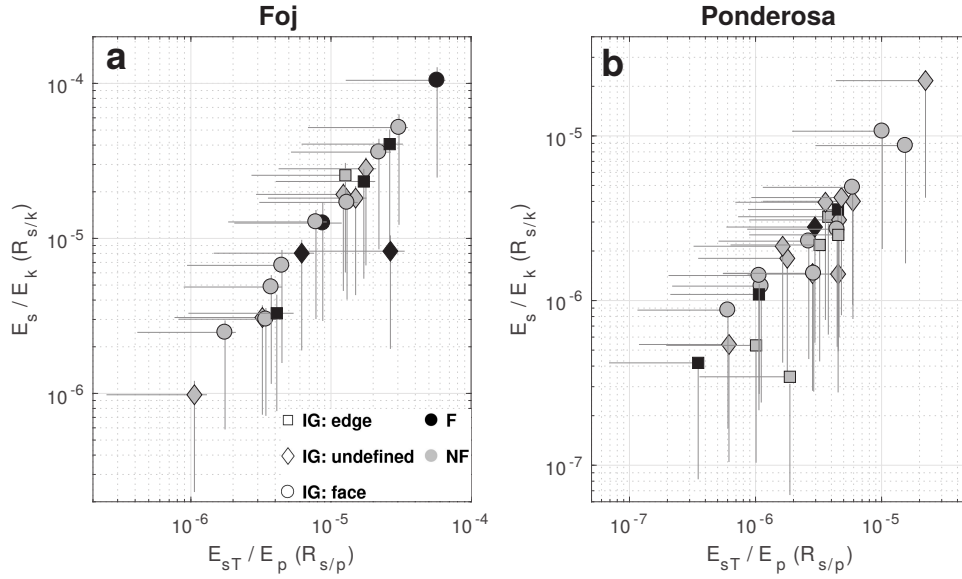
Figure 7. Ratios of seismic energy to potential (X axis) and kinetic (Y axis) energies, for Foj's (a) and Ponderosa's blocks (b). Horizontal and vertical bars in gray show the 5 and 95 th percentiles of the randomized calculation for E_s (shown in Fig. 6) and E_{sT} . The marker's legend is provided below the panels. The marker's edge type corresponds to impact geometry (IG) as determined from the video analysis for each of the released blocks; undefined is indicated when IG could not be determined from the video analysis. Color differentiates F and NF blocks.
