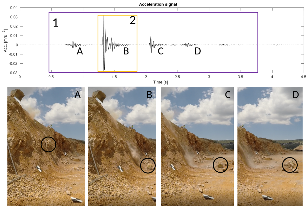
Figure 2. Example of a recorded accelerogram (block 4 at Foj). For each impact, two recordings were kept: the entire signal (1, purple area), and the waveform corresponding to the main impact on the quarry floor (2, orange area). Impact identification was made by comparison with video camera images. See explanations in Sect. 2.1 and 2.2.
