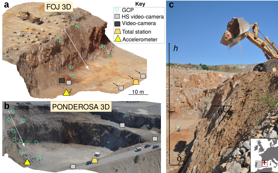
Figure 1. a, b: Images of the 3D models of the testing sites, showing the position of instrumentation. Devices signaled with an arrow were placed in the indicated direction, some steps behind (out of the modelled area). The white arrows indicate the profile section where the block falls took place. The scale is approximate. c: Lateral view of the profile at Foj, indicating the total fall height ( h ), the slope angle ( \theta ), and the considered angle between the deposit and the slope for the volume calculations ( \delta ), according to explanations given in Sect. 3.2 (the same metrics apply to Ponderosa). Note that the testing sites are composed of i. the slope where the fall propagates, and ii. the quarry floor where the main impact of the block takes place, and where the motion of the blocks stops. A small map to contextualize the experiments on a regional scale is also plotted (coordinates provided in Sect. 1).
