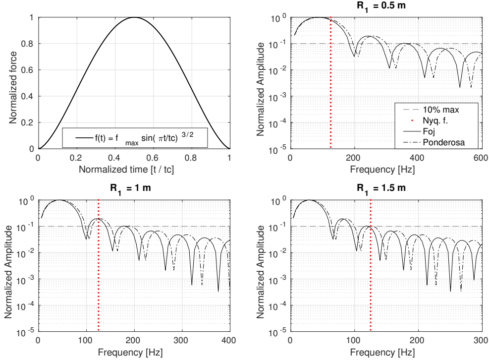
Figure C.1. a: Normalized plot of the simulated force pulse f(t) , and its equation (see text for parameter definitions). Note that, consistent with the rest of the text, normalizations are performed with respect to the maximum value of the variable displayed in the Y axis. In the case of a , the time is also normalized as shown in the figure. b, c, d: Spectrum of the f(t) for three values of R_1 , as obtained for the frequencies of interest. The plots show narrower frequency ranges for larger R_1 s because their amplitude decay increases. The gray discontinuous line serves as the 10% threshold of the maximum spectral velocity amplitude, and the red dotted line represents our Nyquist frequency (i.e. the maximum observable frequency, 125 Hz).
