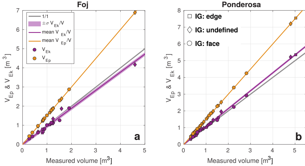
Figure 9. Computed values of V_{Ek} and V_{Ep} , and their relation to measured volumes ( V ). Panel a is for Foj blocks and b is for Ponderosa. The plots also show the mean value of the ratios between the calculated and true volumes, and the standard deviation ( \sigma ) for V_{Ek}/V . The standard deviation of V_{Ep}/V is zero (see text in Sect. 3.2). In this plot, we do not distinguish between fragmented and non-fragmented blocks, and the marker's edge type corresponds to impact geometry (IG), as determined from the video analysis for each of the released blocks; undefined is indicated when IG could not be determined from the video analysis.
