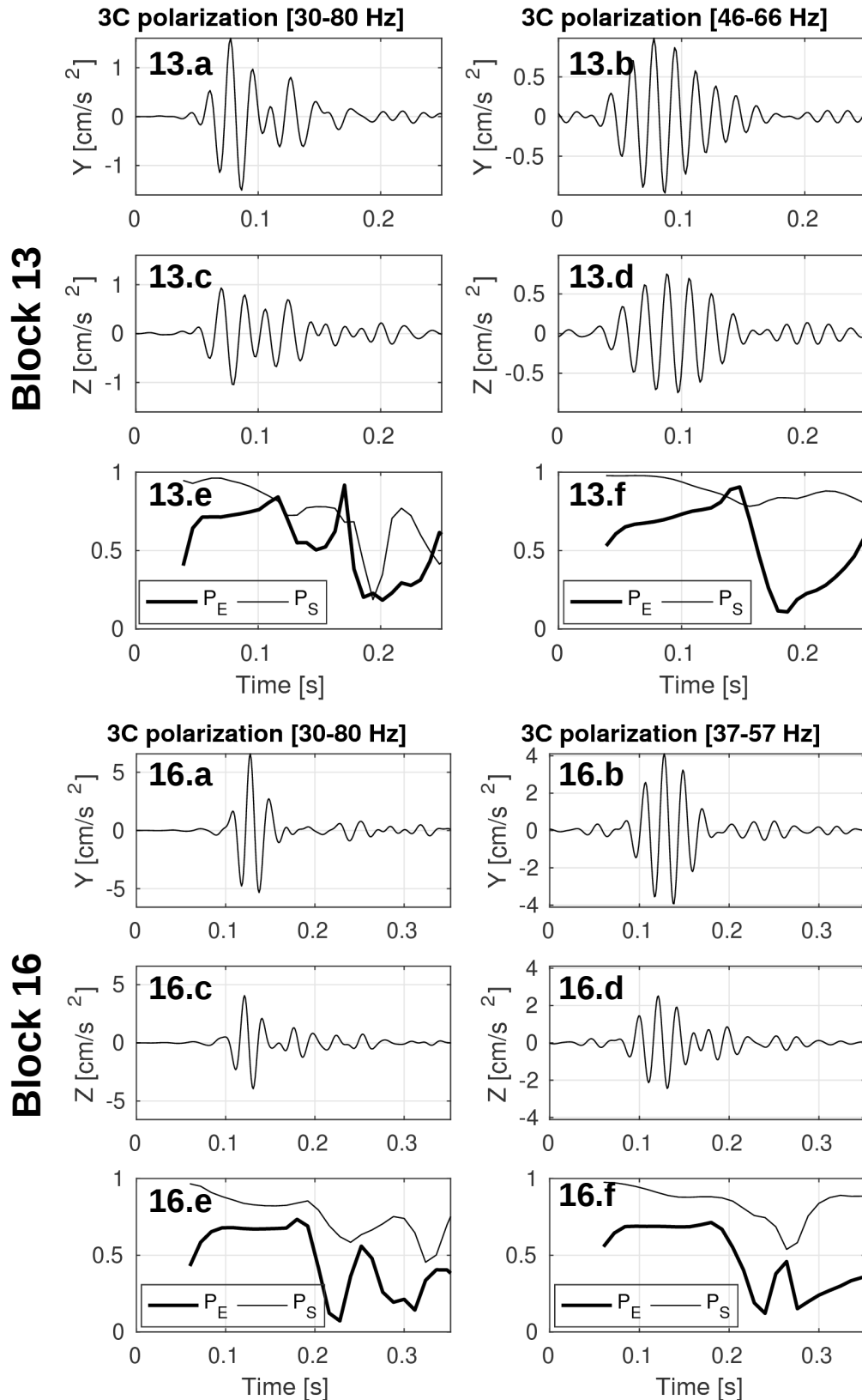
Figure B.1. Results of the 3C polarization analysis for two of the Foj blocks. a, b: Accelerograms corresponding to the maximum component, in this case the radial. c, d: Accelerograms corresponding to the vertical component. e, f: Elliptical component of polarization ( P_E ) and strength of polarization ( P_S ), as obtained for the corresponding recordings. Each column shows signals and polarization results as obtained for the frequency passband indicated at the top. Note that the quantitative analysis employs the three components, even though the transverse is not plotted here. -34-
